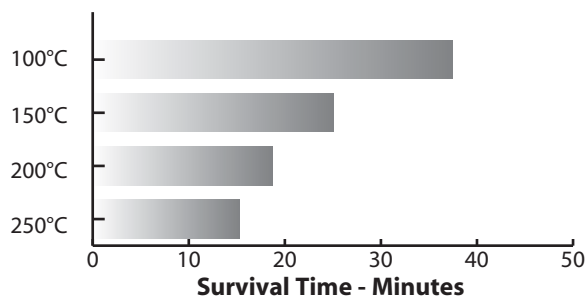
Thermal Protection Duration
