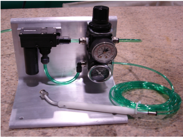
Manual Vacuum Pick and Place device
