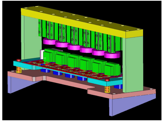
Custom Lead Press & Clinch Tool
